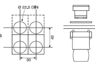
Fixing arrangement
